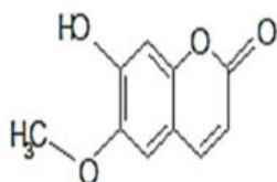
Compound 5: Scopoletin
