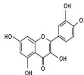
Compound 6: Quercetin
