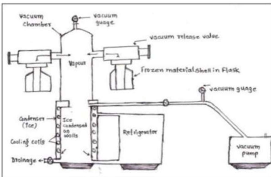
Figure 1: Schematic Diagram of Freeze-drying Technique for Preparation of FDT
